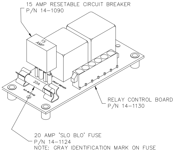
RELAY CONTROL ASSEMBLY P/N 521715 USE WITH GRAY OR YELLOW BOOTED MOTORS
