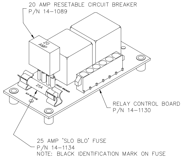
RELAY CONTROL ASSEMBLY P/N 521716 USE WITH BLACK OR RED BOOTED MOTORS
