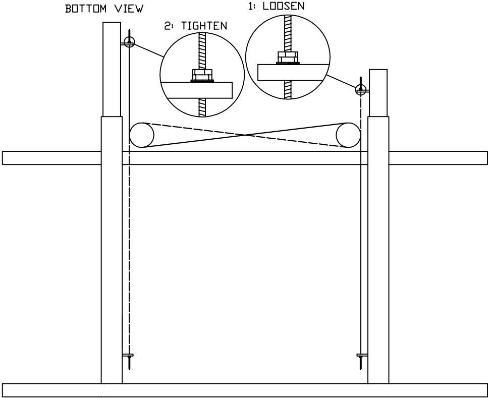
BOTTOM VIEW
