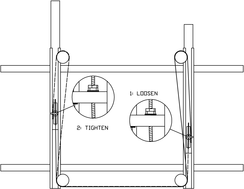
BOTTOM VIEW
