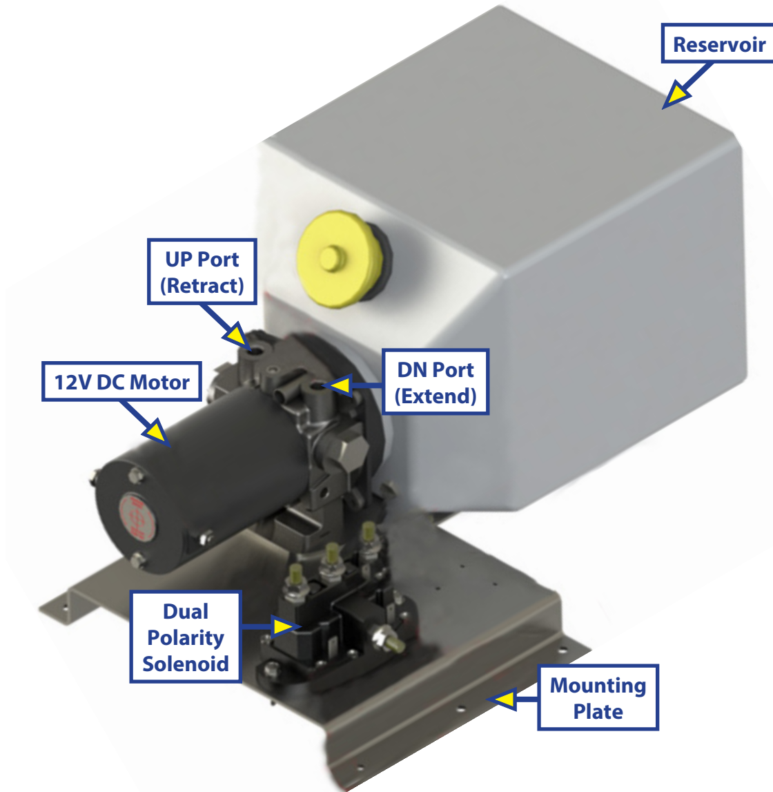
Power Unit - 12V DC Motor with Pump and Reservoir
